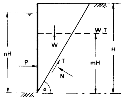
Figure 6.35 Stability of slurry trench.
