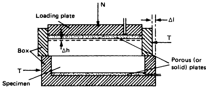
Figure 4.3 Direct shear apparatus.
