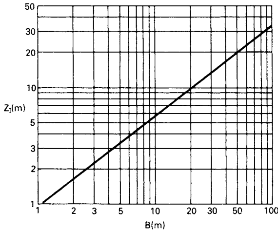
Figure 8.12 Relationship between depth of influence and foundation width. (Reproduced from J.B. Burland and M.C. Burbridge (1985) Proceedings Institution of Civil Engineers, Part 1 , Vol. 78, by permission of Thomas Telford Ltd.)
