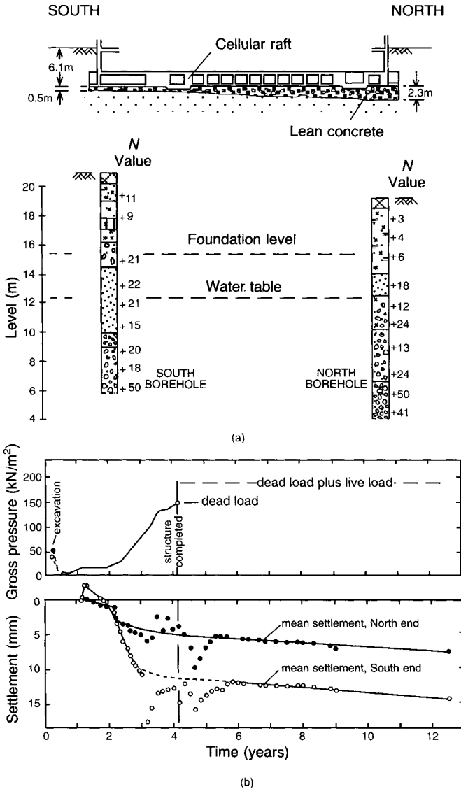
Figure 11.13 Foundation settlement in sand: (a) soil profile and test data and (b) settlement observations. (Reproduced from J.G. Stuart and J. Graham (1975) Settlement performance of a raft foundation on sand , in Settlement of Structures , by permission of Thomas Telford Ltd.)
