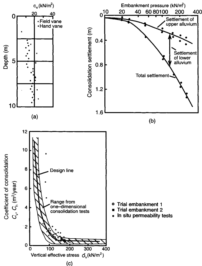
Figure 11.18 Vertical drains: (a) undrained shear strength, (b) pressure-settlement relationships, (c) coefficient of consolidation, (d) field instrumentation and (e) piezometer observations. (Reproduced from J.A. Davies and C. Humpheson (1981) A comparison between the performance of two types of vertical drain beneath a trial embankment in Belfast, Geotechnique , 31 , 19–31, by permission of Thomas Telford Ltd.)
